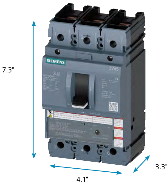
3VA52/62
